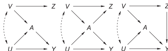
Figure 1. Causal directed acyclic graphs of settings where Z is a negative control outcome (left), a negative control exposure (middle) or both (right). The absence of an arrow denotes the absence of a direct causal link. However, the presence of an arrow need not represent the presence of a direct causal link. Dashed double-headed arrows represent the marginal dependence of the (sets of) variable(s) that they connect, for example, through a common cause.
